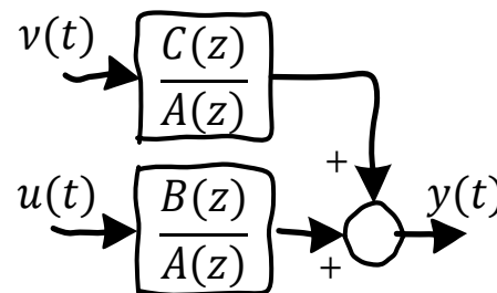
ARMAX
